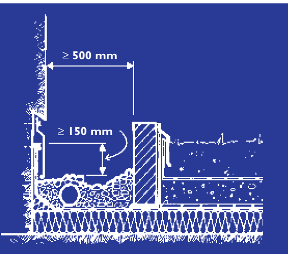
Fig. 10 – Flashing and Gravel Barrier with Drainage Pipe at a Wall/Roof Connection
